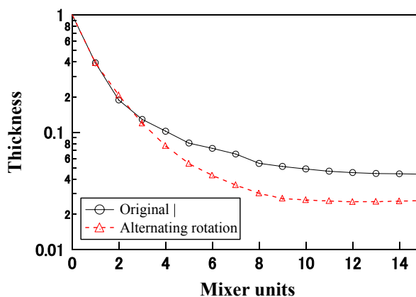
Fig. 14 Average thickness of unmixed islands, 2\langle r \rangle , in the modified mixer ( Re = 1 ).
