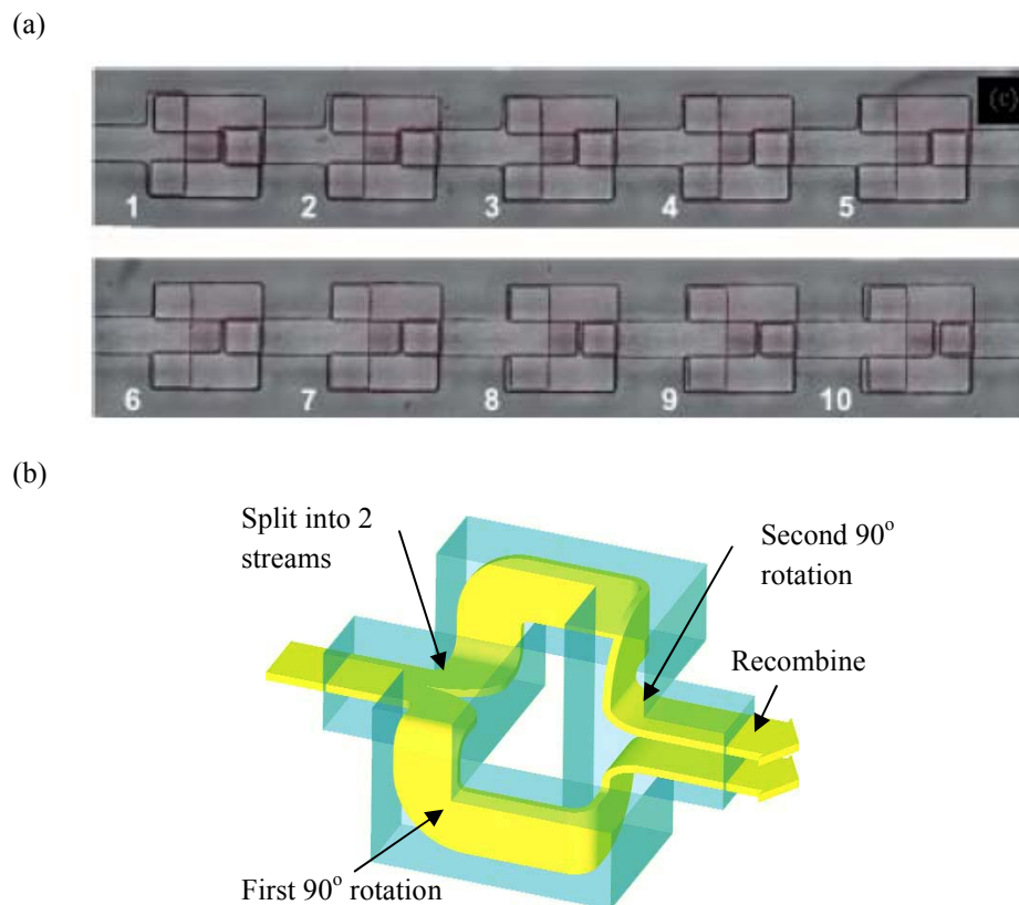
Fig. 2 The SAR micromixer proposed by Tan et al. (9) : (a) fabricated mixer consisting of 10 unit mixers, (b) schematic of a unit mixer.
