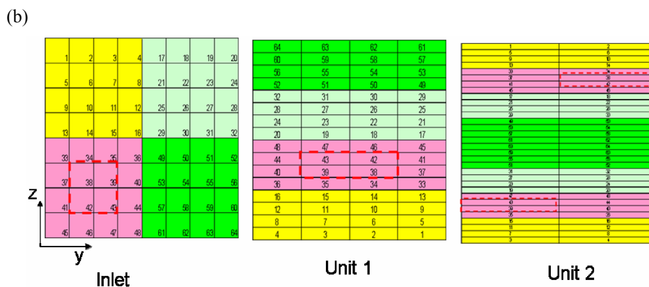
Fig. 4 (a) Movement of the particles initially located in the lower-left region ( Re = 1 ), viewed from the downstream side; (b) expected topology in the ideal lamination.
