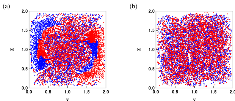
Fig. 7 Distribution of particles in the exit plane of unit 9: (a) Re = 24 ; (b) Re = 66 .
