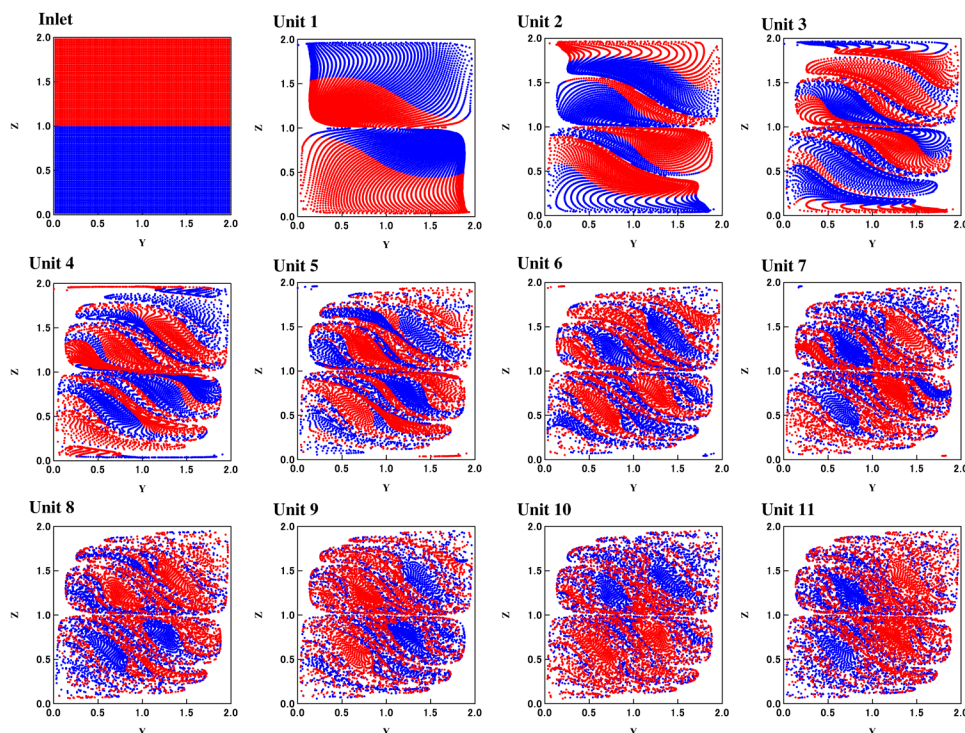
Fig. 3 Distribution of particles at the exit of every mixer unit (i.e., Poincaré section) at Re = 1 , viewed from the downstream side.
